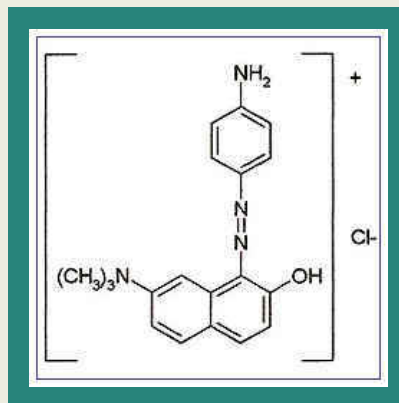
Basic Brown 17
