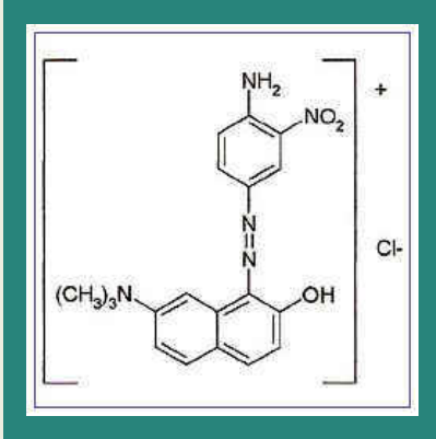
Basic Violet 8
