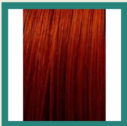
Basic Brown
