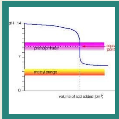
Methyl Orange
