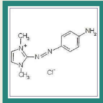
Basic Orange 31
