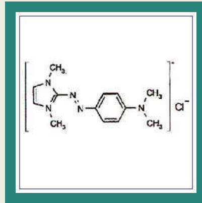
Basic Red 51
