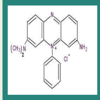
Basic Violet 5
