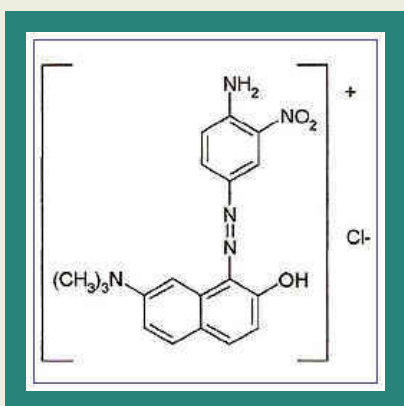
Basic Brown 16
