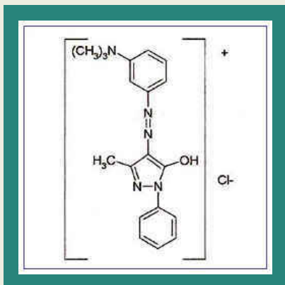
Basic Yellow 57
